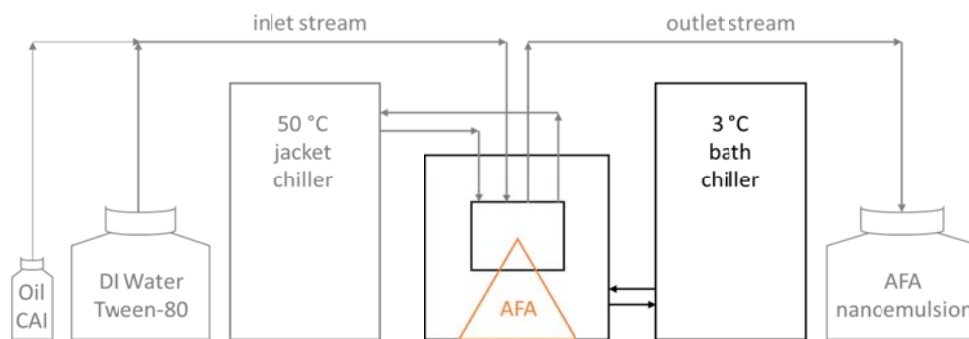
Figure 1. Schematic depicts AFA processing system set up for continuous flow. Oil / CAI stream and water / Tween stream meet before entering flow vessel. Omitting gray portions of diagram reveals batch set up.
