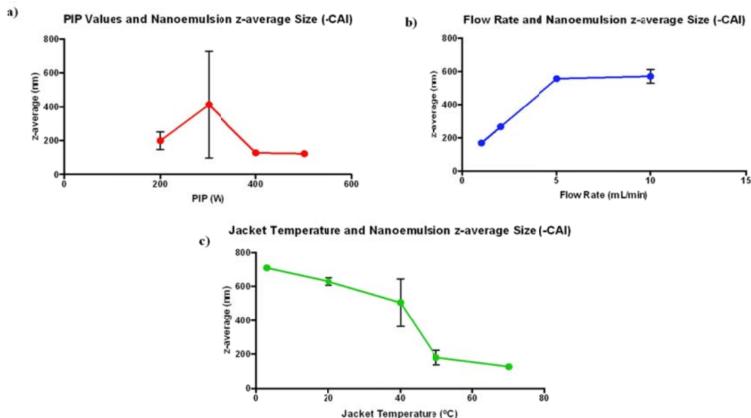
Figure 3. Graphs are scaled separately. All runs lacked CAI. (a) PIP was varied from 200 W to 500 W. Z-average was measured with DLS after 90 minutes of processing. (b) Flow rate was varied from 1 ml/min to 10 ml/min. Z-average was measured after more than 90 ml had been processed. (c) Jacket temperature was varied from 3°C to 70°C. Zetasizer readings were taken after 1 hour.
